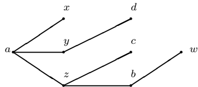
(b): a spanning tree T of K_{4,4} - 4K_2 .
