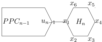
Figure 1: A polyphenyl chain PPC_n with n hexagons, c_n = x_1 and ortho-vertices o_n = x_2, x_6 , meta-vertices m_n = x_3, x_5 , and para-vertex p_n = x_4 in H_n .
