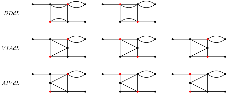
Figure 15: Tiles DDdL , VIAdL , and AIVdL with two independent vertices marked.
