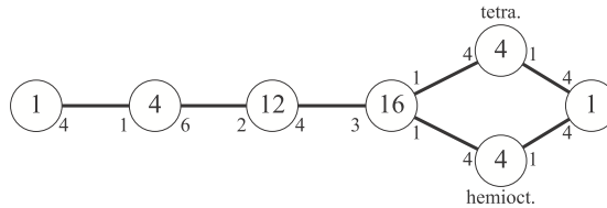
Figure 5: Incidence diagram for the tomotope \mathcal{T} .
