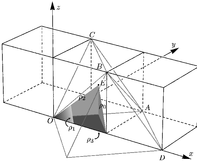
Figure 1: The start of the 4-polytope \mathcal{U} , a uniform tessellation of \mathbb{R}^3 .
