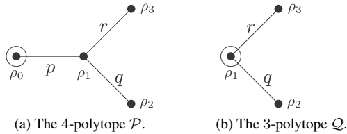
Figure 3: Wythoff’s construction for the 4-polytope \mathcal{P} and its polyhedral vertex-figure \mathcal{Q} .
