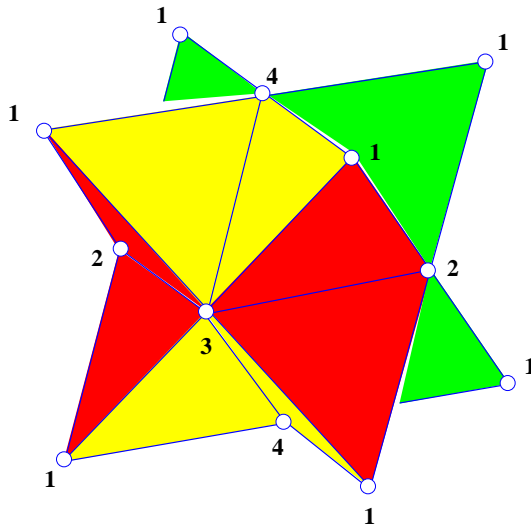
Figure 4: The tomotope \mathcal{T} .
