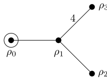
Figure 2: The affine Coxeter group \tilde{B}_3 \simeq \Gamma(\mathcal{U}) .
